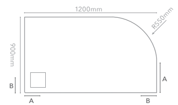
Offset Quadrant Tray
